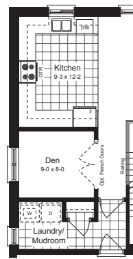
OPTIONAL MAIN FLOOR LAYOUT
