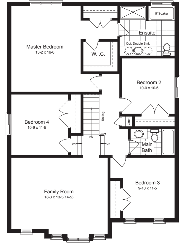
SECOND FLOOR 4 Bedroom Plan
