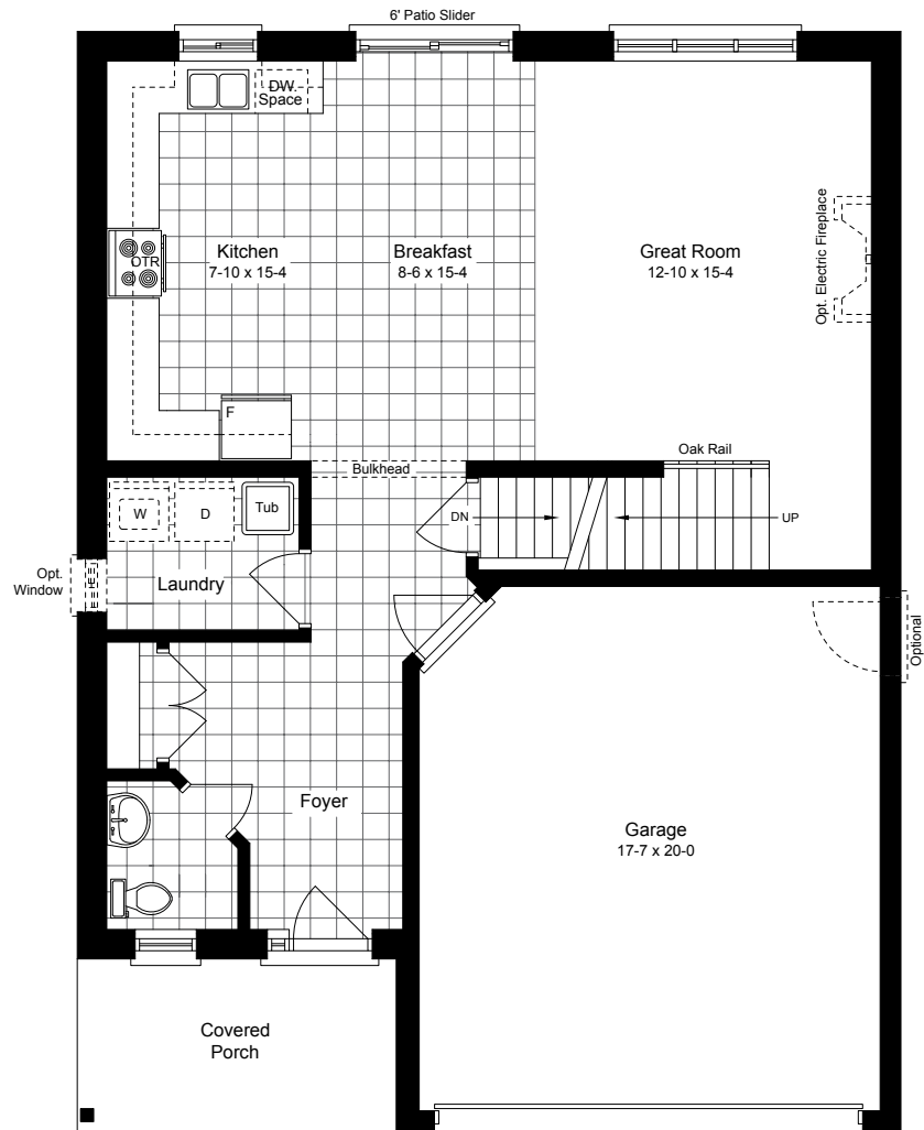
MAIN FLOOR
