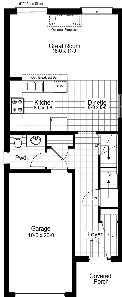
MAIN FLOOR
